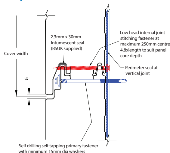
Figure 2. Horizontal joint detail
