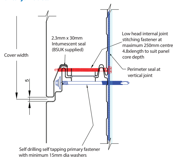
Figure 2. Horizontal joint detail
