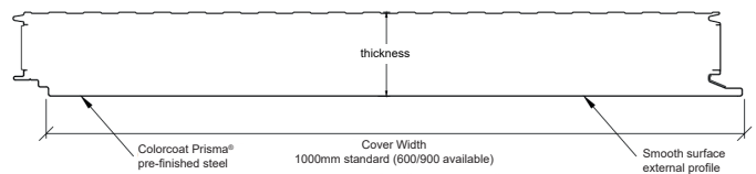
Figure 1. Trimapanel® FW Flat cross section
