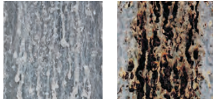
MagiZinc (140gr/m 2 ) and Zinc (275gr/m 2 ) after 5 weeks in salt spray test
