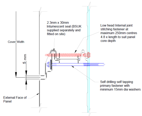
Figure 2. Formawall® FW system fixing detail
