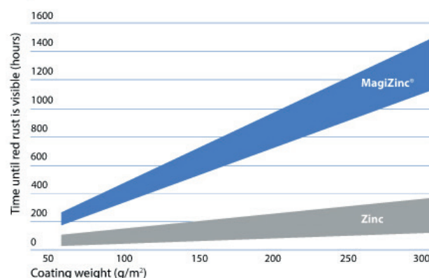
Salt spray testing (accelerated corrosion) of MZ and Zinc metallic coatings
