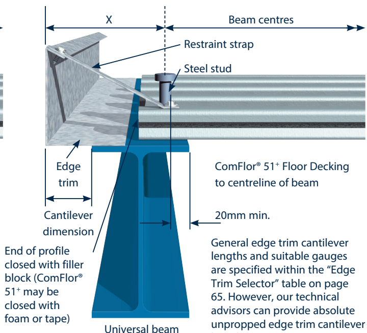
End detail alternative 2
