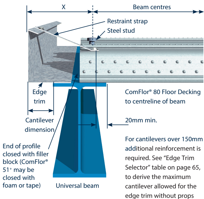
End detail
