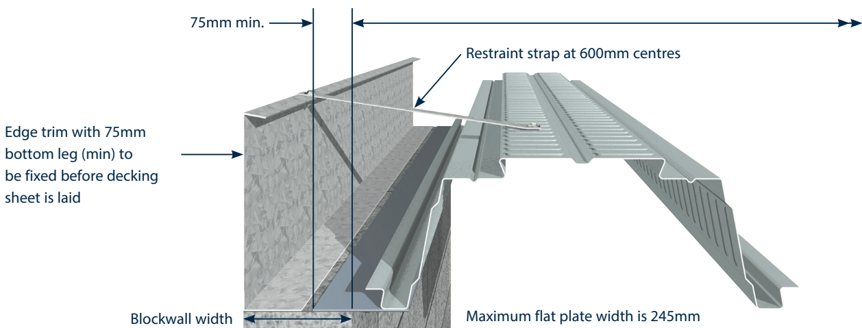
Cut plate on blockwork
