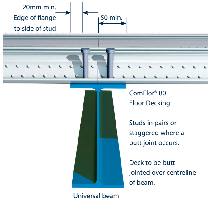
Butt joint
