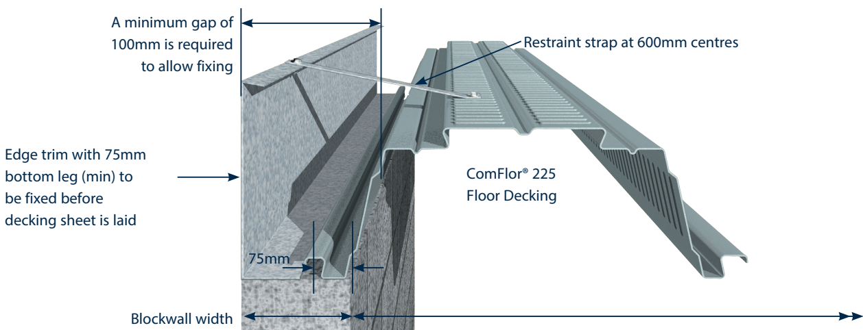
Side fixing onto blockwork
