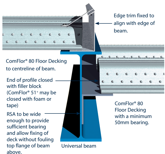
Step in floor
