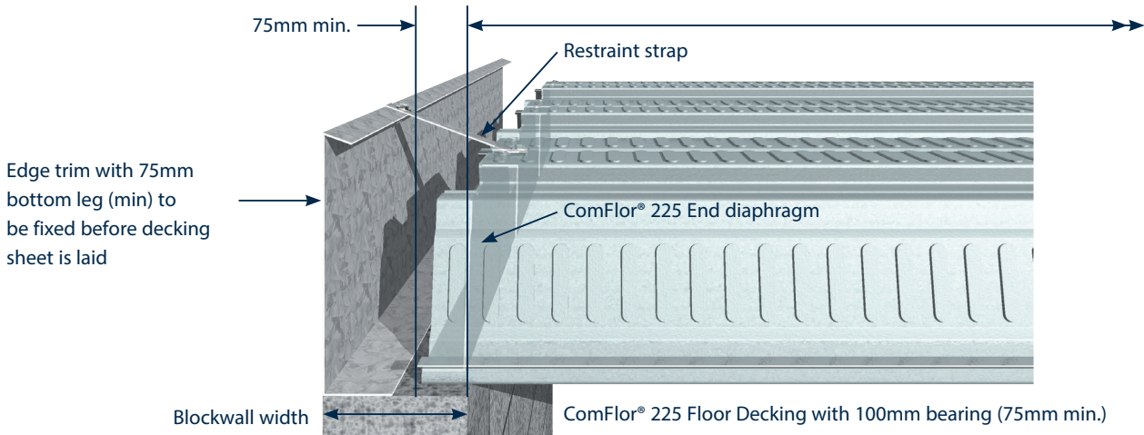
End fixing onto blockwork
