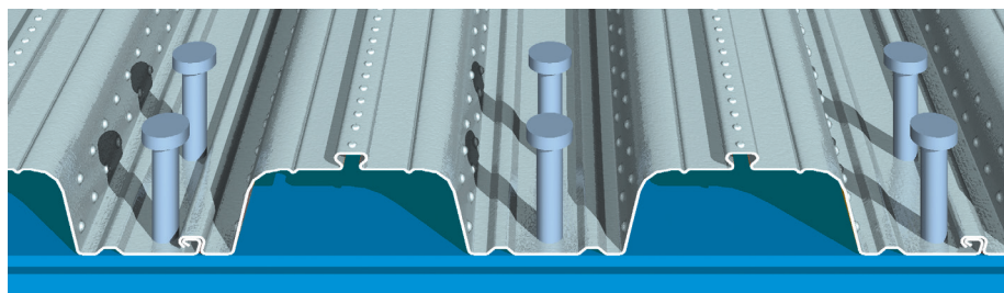
CENTRAL STUDS
