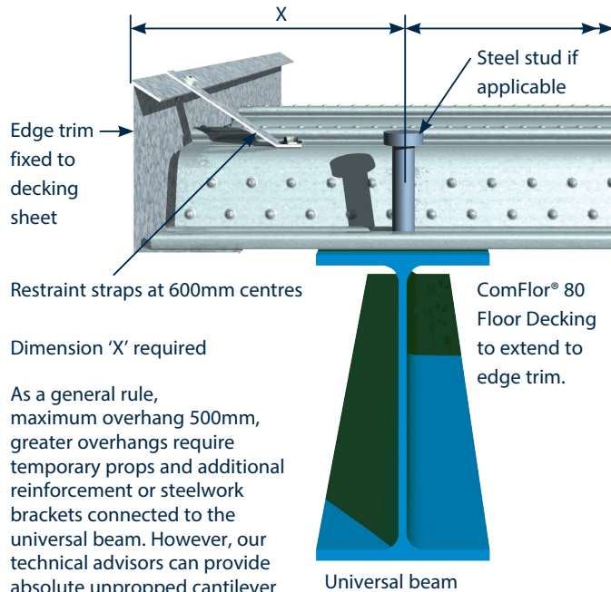
Typical end overhang
