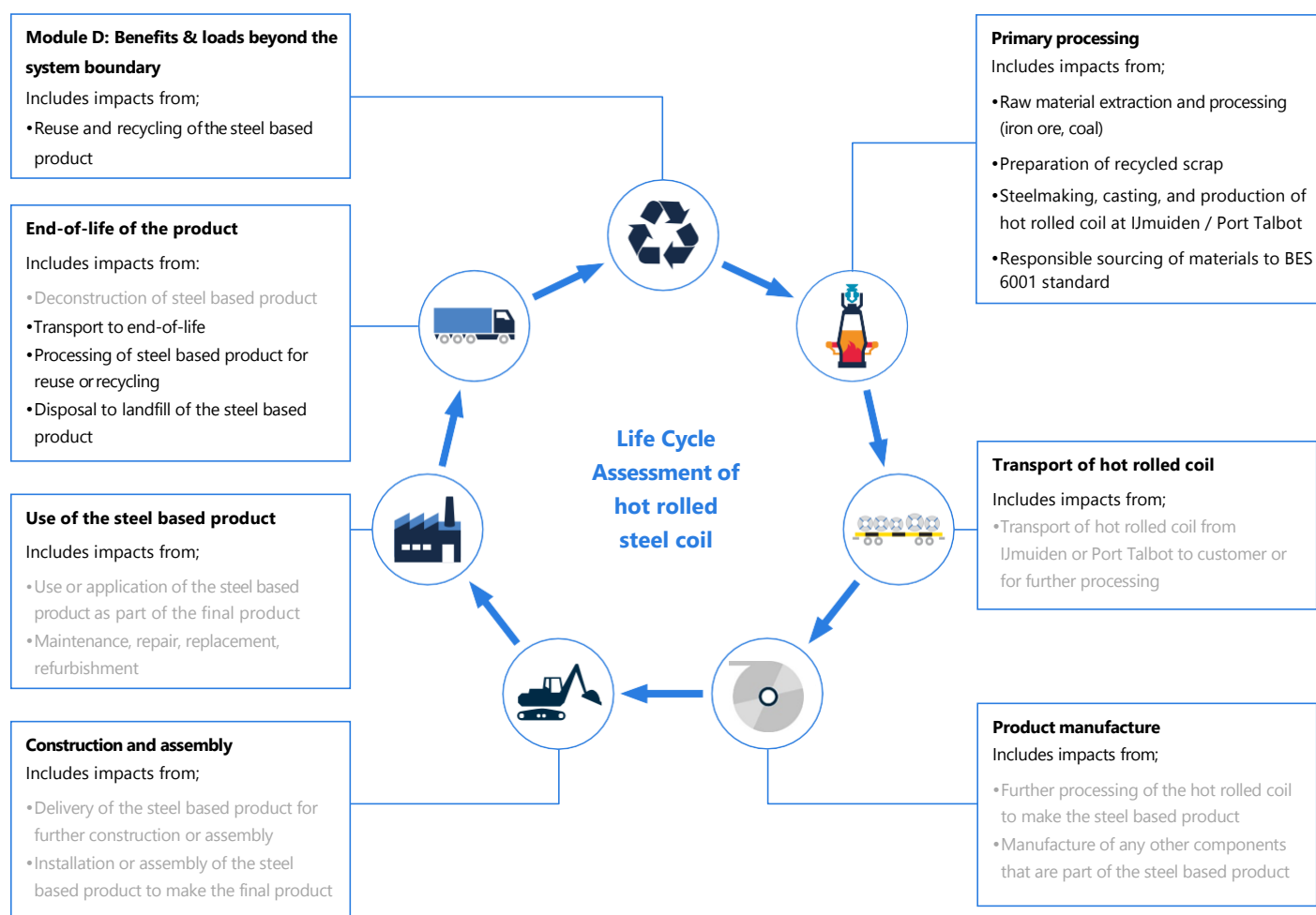
Figure 2 Life Cycle Assessment of steel hot rolled coil
