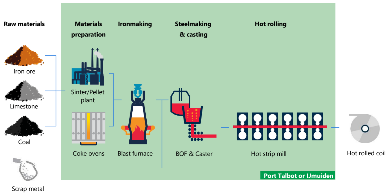
Figure 1 Process overview from raw materials to hot rolled coil
