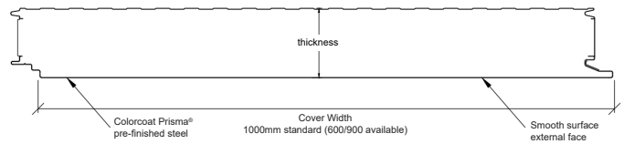
Figure 1. Trimapanel® Flat cross section
